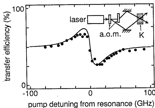
FIG. 2. Energy-transfer efficiency, defined as the ratio of the output energy of the probe wave to the total input energy, as a function of the pump-wave detuning from resonance. The experimental setup is shown in the inset (a.o.m. is the acousto-optic modulator, K is the potassium vapor cell). The pump and probe waves have equal input energies of 20 \mu\text{J} , the detuning of the probe wave from the pump wave is \delta/2\pi = 3 \text{ MHz} , and the temperature of the body of the potassium cell is 220^\circ\text{C} . The solid curve gives the best theoretical fit to the experimental data.
