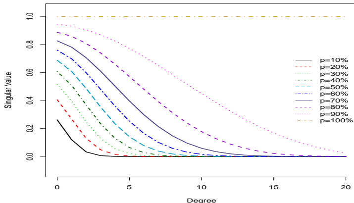
FIG 2. Singular values decay under Induced Subgraph sampling. M = 20 .
