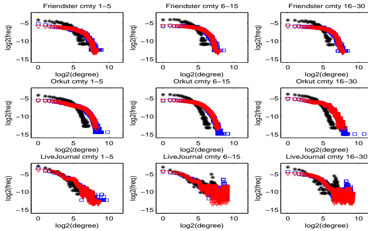
FIG 10. Estimating degree distributions of communities from Friendster, Orkut and LiveJournal. Squares represent the true degree distributions, dots represent the sample degree distributions, triangles represent the estimated degree distributions. Sampling rate=30%. Points which correspond to a density < 10^{-4} are eliminated from the plot. (Online versions of figure are in color.)
