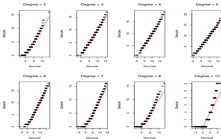
FIG 6. QQ plot: distribution of N_i^* compared to Gaussian distribution with mean (PN)_i and sample variance. The underlying network is ER with n_v = |V| = 1000 and n_e = |E| = 50000 . Sampling rate p = 5\% . The average degree of sample is equal to 5.
