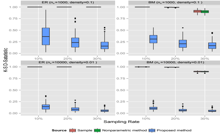
FIG 9. Simulation results for induced subgraph sampling. Error measured by K - S D -Statistic. For each sampling rate, the three boxes from left to right represent K - S D -Statistic comparing the true degree distribution with (left) sample degree distribution, (middle) estimated degree distribution using the non-parametric method, and (right) estimated degree distribution using the proposed method. (Online versions of figure are in color.) (Note: Only the performance of the proposed estimator \hat{N} avoids the extremes of 1.0 in most cases.)
