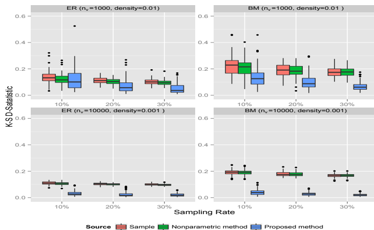
FIG 8. Simulation results for one-wave snowball sampling. Error measured by K - S D -Statistic. For each sampling rate, the three boxes from left to right represent K - S D -Statistic comparing the true degree distribution with (left) sample degree distribution, (middle) estimated degree distribution using the non-parametric method, and (right) estimated degree distribution using the proposed method. (Online versions of figure are in color.)
