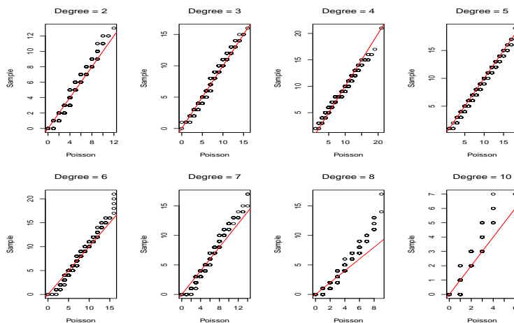
FIG 5. QQ plot: distribution of N_i^* compared to Poisson distribution with mean (PN)_i . The underlying network is ER with n_v = |V| = 1000 and n_e = |E| = 50000 . Sampling rate p = 5\% . The average degree of sample is equal to 5.
