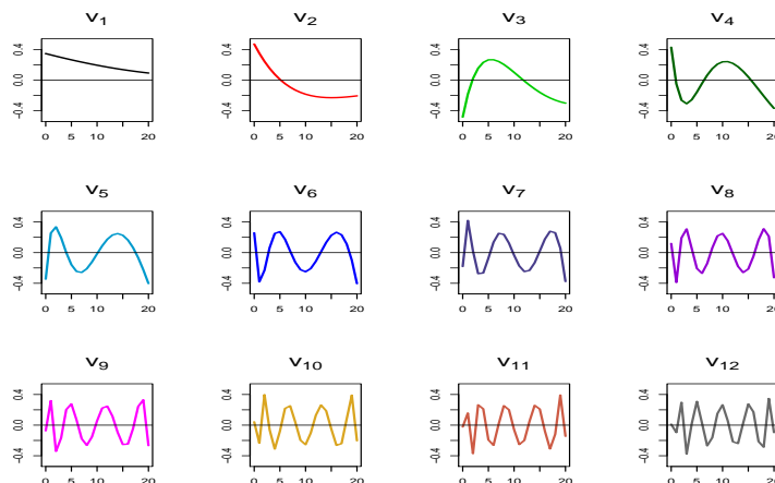
FIG 3. The first 12 right singular vectors under Induced Subgraph sampling, ordered by singular values from big to small: maximum degree M = 20 , sampling rate p = 20\% .
