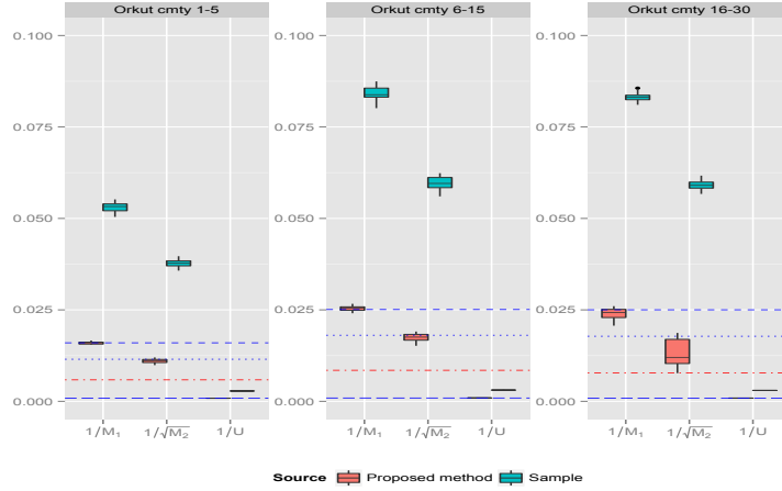
FIG 12. Bounds for the epidemic spreads of Orkut networks, each box is estimated based on 20 samples, four horizontal lines are the true values for \frac{1}{M_1} , \frac{1}{\sqrt{M_2}} , \frac{1}{\lambda_1} and \frac{1}{U} from top to bottom. For each bound, the two boxes from left to right correspond to the estimated value using (left) the proposed method and (right) the sample degree distribution. (Online versions of figure are in color.)
