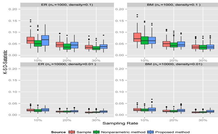
FIG 7. Simulation results for ego-centric sampling. Error measured by K-S D-Statistic. For each sampling rate, the three boxes from left to right represent K-S D-Statistic comparing the true degree distribution with (left) sample degree distribution, (middle) estimated degree distribution using the non-parametric method, and (right) estimated degree distribution using the proposed method. (Online versions of figure are in color.)
