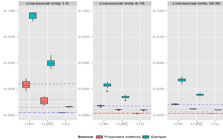
FIG 13. Bounds for the epidemic spreads of LiveJournal networks, each box is estimated based on 20 samples, four horizontal lines are the true values for \frac{1}{M_1} , \frac{1}{\sqrt{M_2}} , \frac{1}{\lambda_1} and \frac{1}{U} from top to bottom. For each bound, the two boxes from left to right correspond to the estimated value using (left) the proposed method and (right) the sample degree distribution. (Online versions of figure are in color.)
