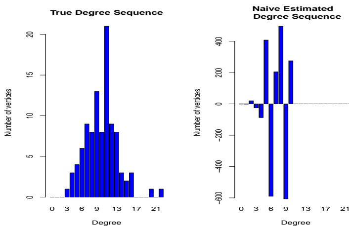
FIG 1. Left: ER graph with 100 vertices and 500 edges. Right: Naive estimate of degree distribution, according to equation (2.2). Data drawn according to induced subgraph sampling with sampling rate p = 60\% .
