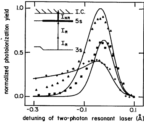
FIG. 2. Excitation spectra for several nonresonant laser intensities: pluses, 4.2 \text{ GW cm}^{-2} ; triangles, 0.42 \text{ GW cm}^{-2} ; squares, 0.067 \text{ GW cm}^{-2} . The inset shows the relevant atomic energy levels and laser fields. The ground state is Stark shifted and the intermediate level is broadened as a result of both two-photon absorption and excitation to the ionization continuum (I.C.).
