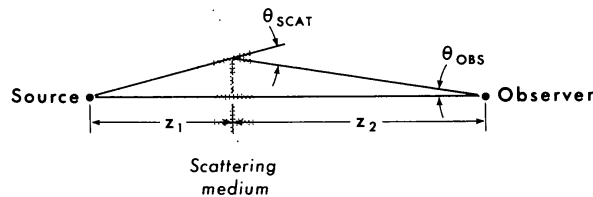
FIG. 1.—Scattering geometry showing relation between \theta_{\text{scat}} and \theta_{\text{obs}}
