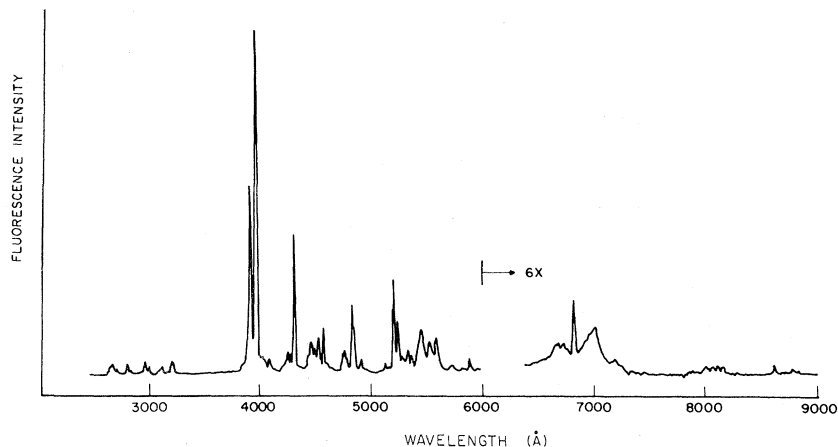
FIG. 3. Spectrum of the emission excited by three-photon absorption at an excitation wavelength of 5935 Å.
