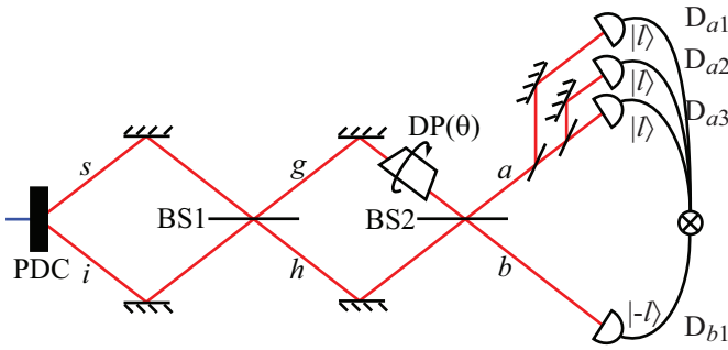
FIG. 3: A scheme for supersensitive measurement of angular displacement using four entangled photons. \theta is the angle of rotation of the Dove prism in mode g . D_{a1} , D_{a2} , D_{a3} and D_{b1} are detectors set to detect one photon each in the mode characterized by index l , l , l , and -l , respectively.
