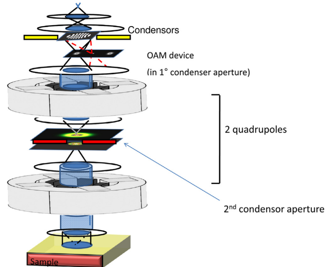
Fig. 6. Second proposed scheme to generate a spin-polarized electron beam based on coupling with two magnetic quadrupoles (spherical aberration corrector). The second quadrupole corrects the aberration induced by the first one. Nevertheless, the spin-to-orbit coupling efficiency after the second quadrupole can be completely neglected.
