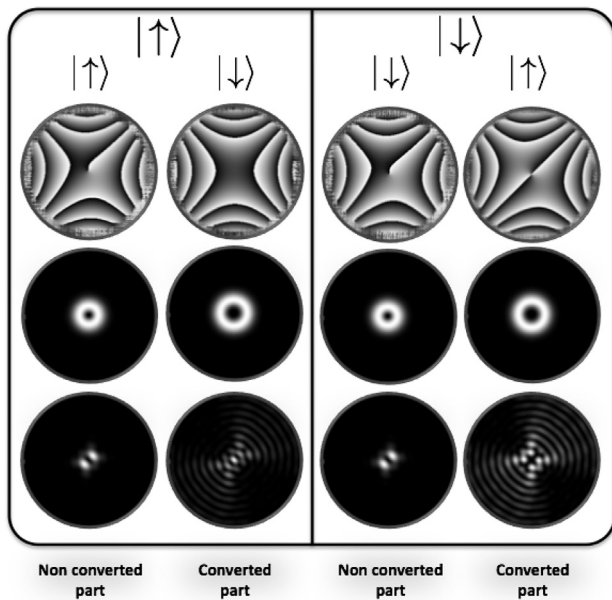
Fig. 7. As the beam with OAM = +1 propagates inside the aberration corrector system (quadrupole–condenser–aperture and a rotated quadrupole), it sees an astigmatism effect introduced by the quadrupoles and, based on the time interaction, a portion of electrons undergo spin-to-orbit conversion (second and fourth column). The first two rows show phase and intensity distributions of the electron beam after the first quadrupole for a mixture of 50–50 spin up and down, respectively. The last row shows output intensity distributions for both the converted and non-converted parts of spin up and down after interacting with the whole system. The simulation was carried out for an input electron beam size of 1\ \mu\text{m} , a quadrupole magnetic field of 0.1\ \text{mT} at the beam waist radius, and a device thickness of 10\ \mu\text{m} . This relatively small thickness was chosen to simplify and speed up the numerical calculation and to avoid too large phase deformations.
