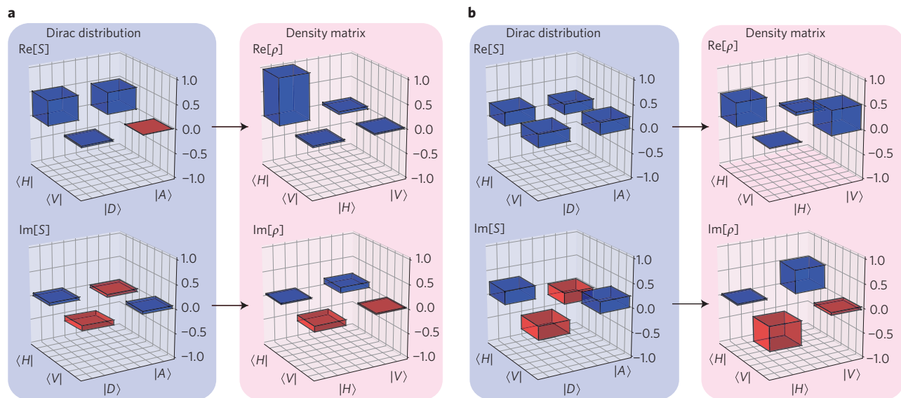
Figure 4 | Results of experiment 2. a,b , The directly measured Dirac distributions (left) and corresponding density matrices (right) for the horizontal linear polarization state |H\rangle ( a ) and left-hand circular polarization state |L\rangle = 1/2(1 + i)|H\rangle + (1 - i)|V\rangle ( b ). The axes of the Dirac distribution are the mutually unbiased bases H/V and D/A ; the density matrix describes the state in terms of only one basis, H/V . Red towers indicate negative values.
