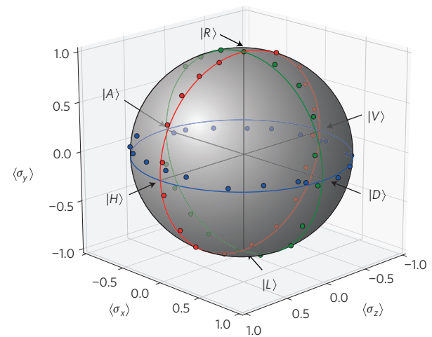
Figure 3 | Measured states on the Poincaré sphere. A Poincaré sphere with the set of directly measured states, indicated by their calculated Stokes parameters \langle\sigma_x\rangle = \langle\psi|(\pi_D - \pi_A)|\psi\rangle , \langle\sigma_y\rangle = \langle\psi|(\pi_R - \pi_L)|\psi\rangle , \langle\sigma_z\rangle = \langle\psi|(\pi_H - \pi_V)|\psi\rangle . Blue points indicate states created by rotating the half-wave plate. Red (green) points indicate calculated Stokes parameters for states created by rotating the half-wave plate, followed by a quarter-wave plate at fixed angle of 0^\circ ( 45^\circ ). Solid lines indicate paths taken for each data set.
