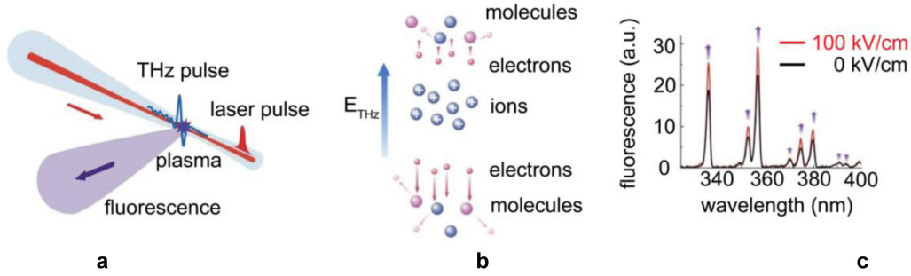
FIG. 5: (a) Experimental geometry for THz-REEF from air-plasma using a single-color laser pulse. (b) Electron acceleration in the THz field and collision with neighboring molecules. (c) THz-enhanced fluorescence spectra of nitrogen gas-plasma under influence of 100 kV/cm peak field.
