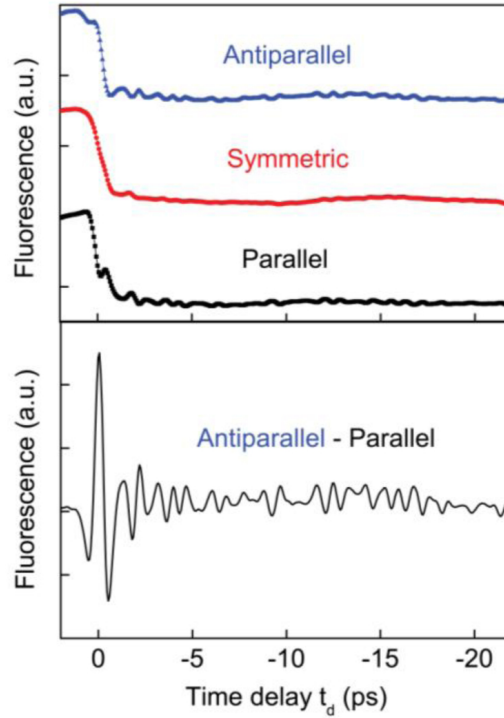
FIG. 6: Time-resolved air-plasma fluorescence enhancement from THz wave interaction with antiparallel, symmetric, and parallel electron drift velocities with respect to the laser field, controlled by changing the relative phase between the \omega and 2\omega optical pulses. Subtracting the parallel curve from the antiparallel curve removes the incoherent energy transfer by electrons after inelastic collisions and scattering at random directions. This reveals the THz waveform in the form of fluorescence modulation. The optical pulse leads the THz pulse in time for delay t_d < 0 .
