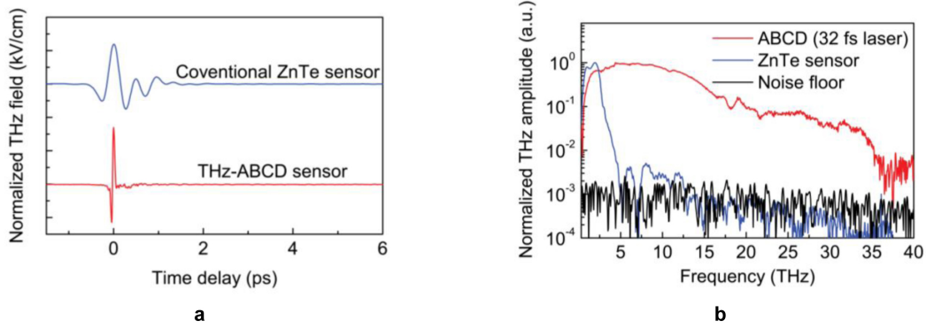
FIG. 3: (a) Time-resolved THz signals generated and detected using dry nitrogen gas as compared to conventional EO crystal detection in ZnTe. The probe beam for air detection has energy of 85 \mu J and pulse duration of 32 fs. (b) Corresponding spectra after Fourier transform.
