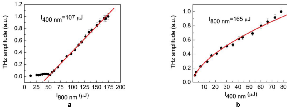
FIG. 2: Dependence of THz field on fundamental ( \omega ) pulse energy, with fixed second-harmonic ( 2\omega ) pulse energy. (b) Dependence of THz field on second-harmonic pulse energy, with fixed fundamental pulse energy. The solid line and curve are the linear and square-root fits, respectively.
