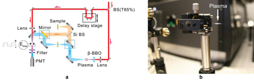
FIG. 1: Schematic diagram of a THz-ABCD spectroscopic system in both transmission and reflection mode. The system can be converted from transmission to reflection mode by taking off the mirrors indicated with an enclosing dashed box. (b) Photograph of laser-induced air-plasma created after focusing the optical beam from left to right through a lens (left) and mounted nonlinear crystal (center) used for second harmonic generation. The bright horizontal line emits an intense, highly directional THz field to the right. PMT: photomultiplier tube; BS: beamsplitter; \beta -BBO: beta-barium borate.
