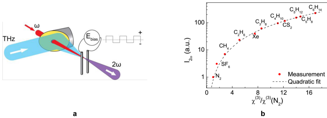
FIG. 4: (a) Basic concept of THz-ABCD: electrodes are placed at the geometric focus of collinearly focused THz and optical probe beams with a variable time delay. Second harmonic light is induced from the THz field and the local bias field E_{bias} . Modulating E_{bias} allows for heterodyne detection for enhanced sensitivity. (b) Measured second harmonic intensity vs. third order nonlinear susceptibility \chi^{(3)} . All \chi^{(3)} are normalized with respect to nitrogen.
