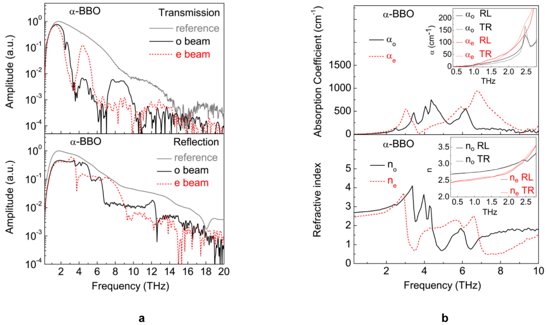
FIG. 10: (a) Measured transmitted and reflected THz spectra of a 0.3-mm-thick \alpha -BBO crystal and reference spectrum. (b) Absorption coefficients and refractive indices of the \alpha -BBO for both e and o crystal axis in the range of 0.3–10 THz. (Insets) Comparison between transmission (TR) and reflection (RL) measurements.
