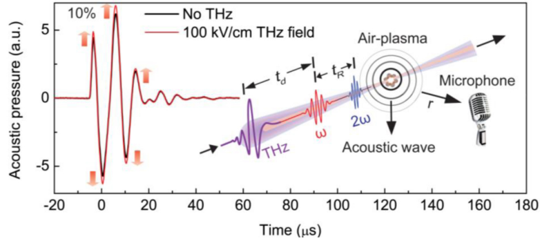
FIG. 8: Single acoustic pulse measured using a high frequency microphone from 10 mm radial distance when an 85 fs, 100 \mu J optical pulse is focused into air with and without interaction with THz radiation. (Inset) Schematic of a THz-enhanced acoustics (TEA) measurement. A pulsed laser and its second harmonic generate an air-plasma which releases acoustic waves that are enhanced under the influence of THz radiation. A microphone detects the amplitude changes in these pressure waves.
